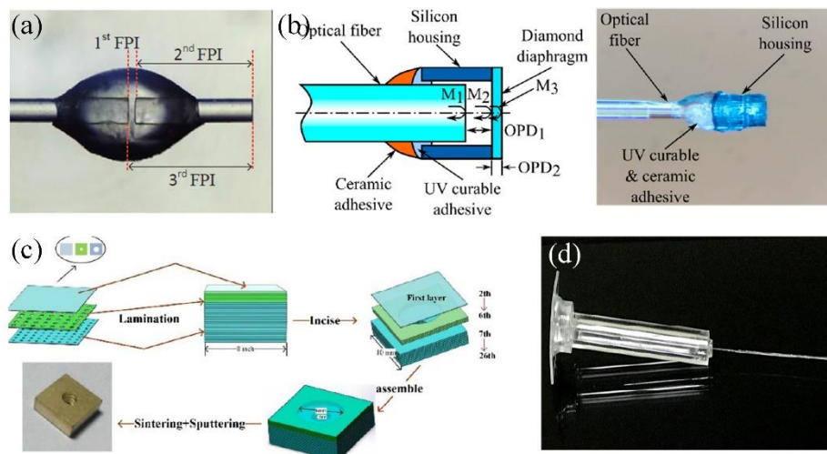
Fig. 5 (a)-(b) Optic-fiber FP pressure sensor fabricated by bonding technology
