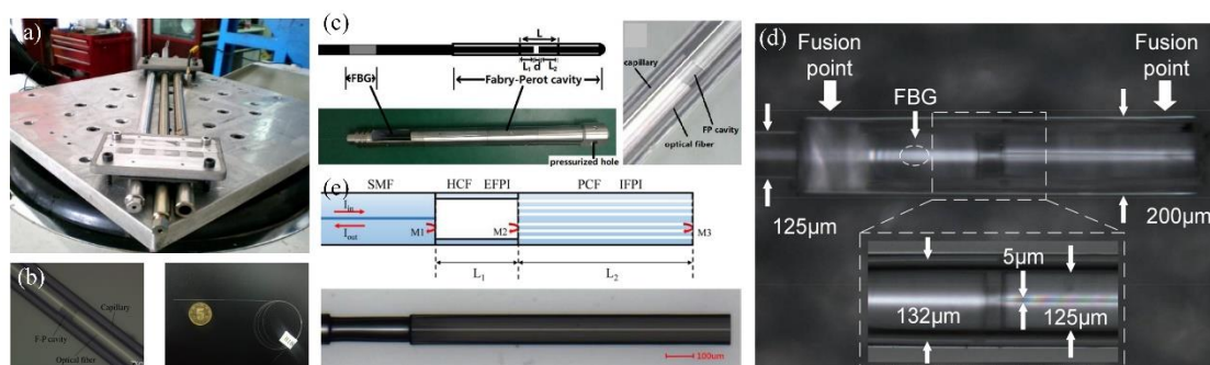
Fig. 4 (a)-(e) Optic-fiber FP pressure sensor fabricated by fusion splicing technology.
