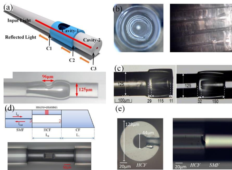
Fig. 3 (a)–(e) Optic-fiber FP pressure sensor made by laser processing technology.
