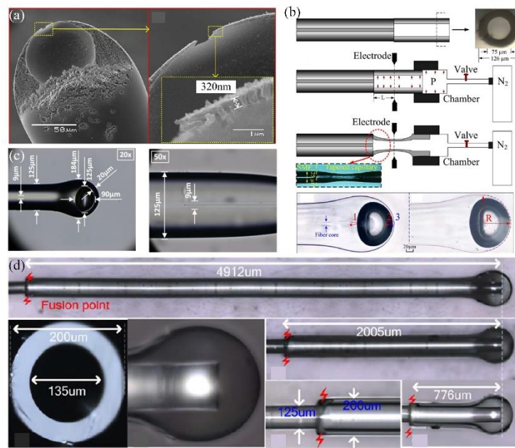
Fig. 1 (a)–(d) Optic-fiber FP Pressure Sensor fabricated by arc discharge technology.
