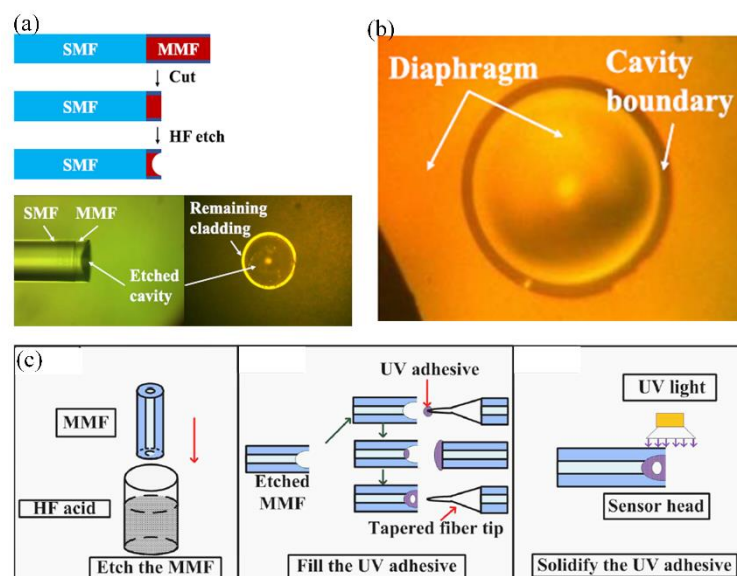
Fig. 2 (a)–(c) Optic-fiber FP pressure sensor fabricated by chemical etching technology.
