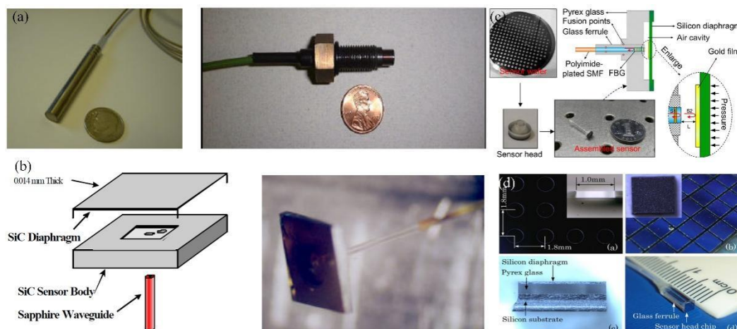
Fig. 6 (a)-(b) Optic-fiber FP pressure sensor based on Si and SiC developed by Luna Company (c) Optic-fiber FP pressure sensor developed by North University of China (d) Optic-fiber FP pressure sensor developed by Tianjin University.
