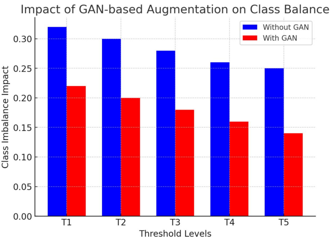
Figure 2 illustrates the impact of GAN-based augmentation and cost-sensitive learning on addressing class imbalance, highlighting improvements in recall and risk assessment precision.
