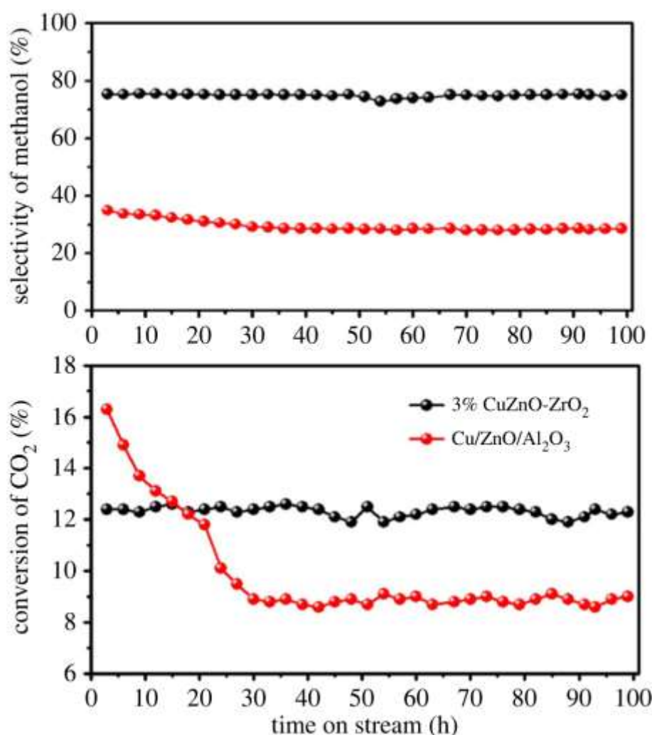
Figure 2 CO 2 conversion and methanol selectivity measured at different catalyst compositions and temperatures for Cu-doped ZnO–ZrO 2 catalysts.
