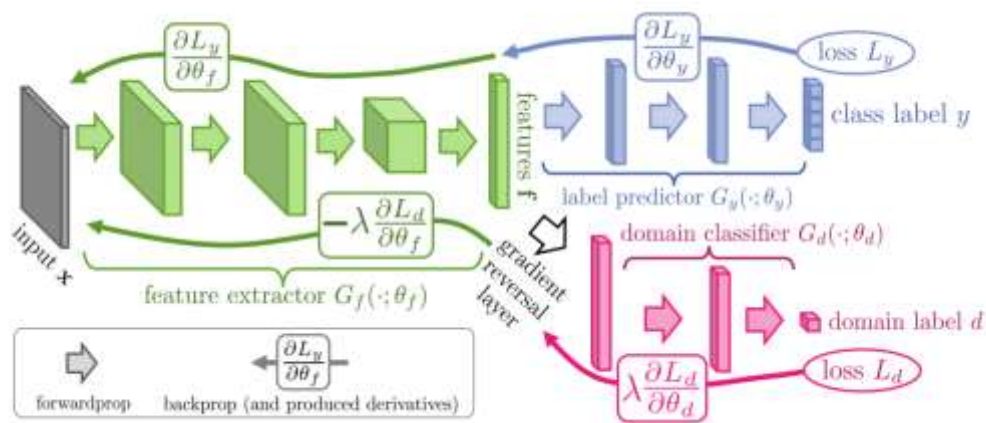
Figure 1. Feature Extractor
