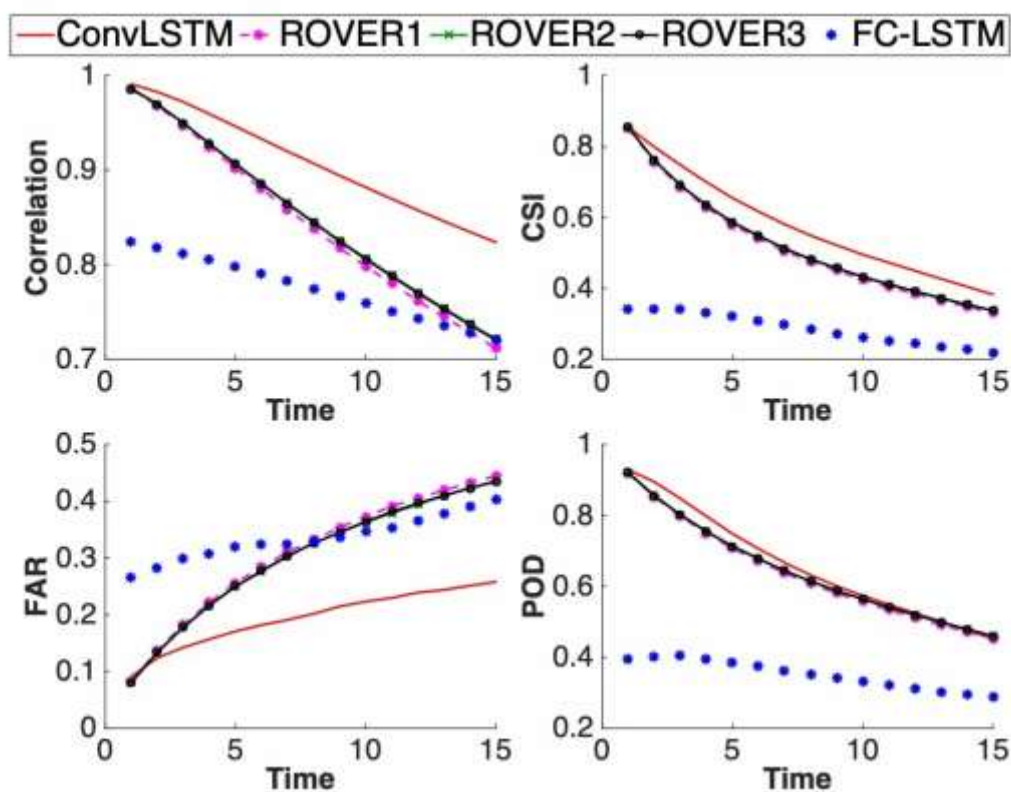
Figure 3 Multi-horizon prediction performance comparison across model architectures evaluated on the regional transformer failure test set
