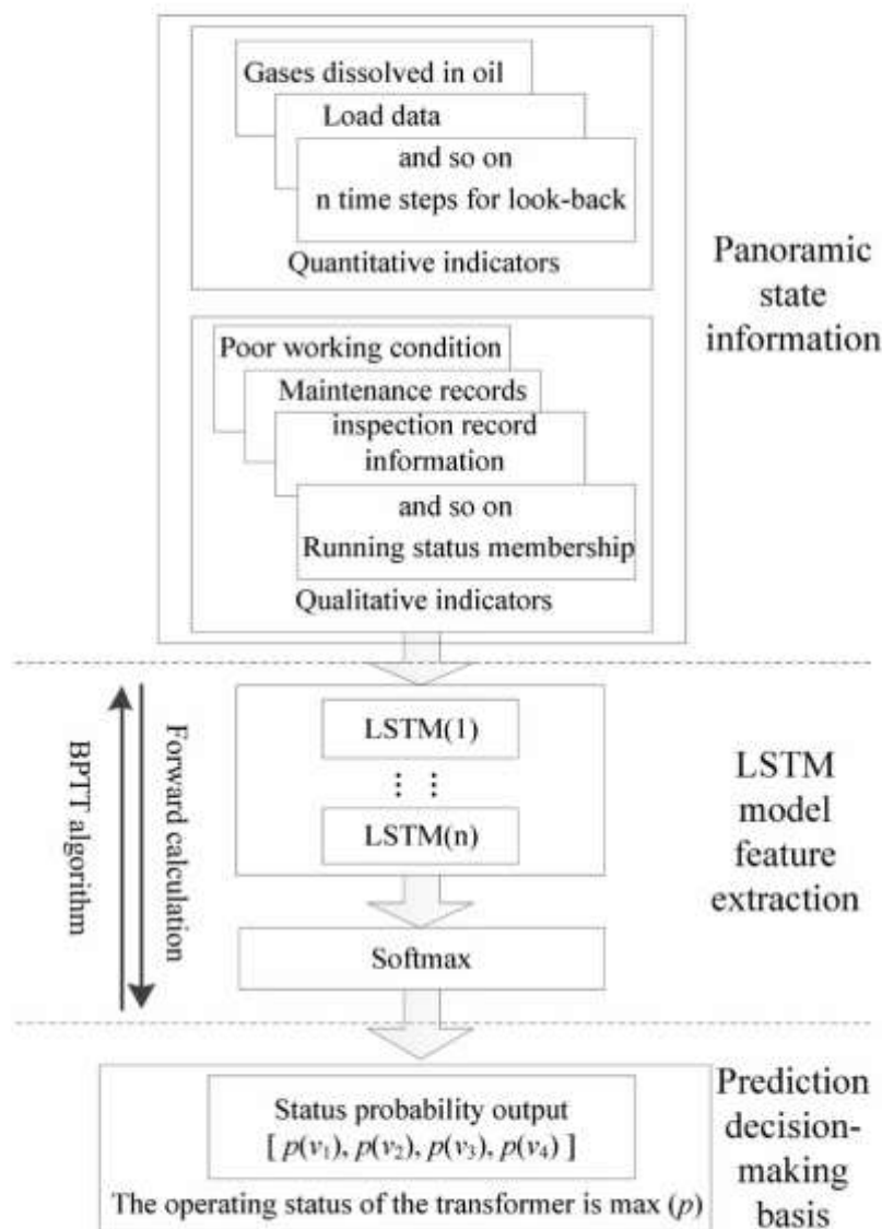
Figure 2 Panoramic state information processing pipeline for individual transformer nodes in the proposed framework
