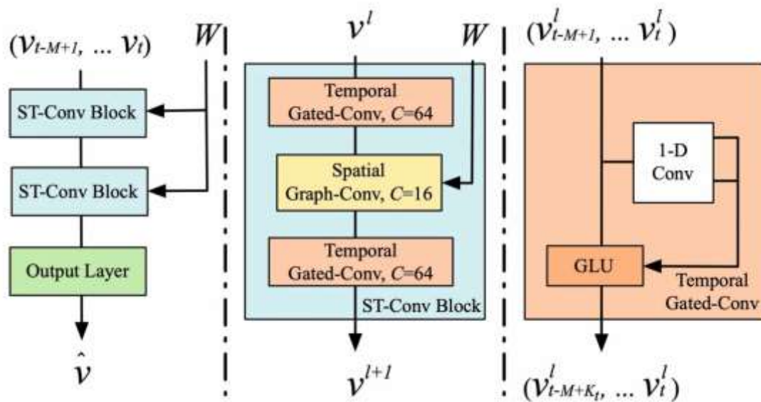
Figure 1 Architecture of the Spatio-Temporal Graph Convolutional Network used in the proposed transformer failure prediction framework
