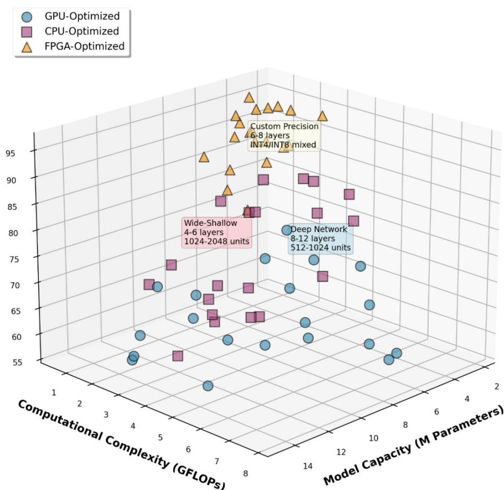
Figure 2: Architecture Search Space and Discovered Architectures for Cross-Hardware Deployment
