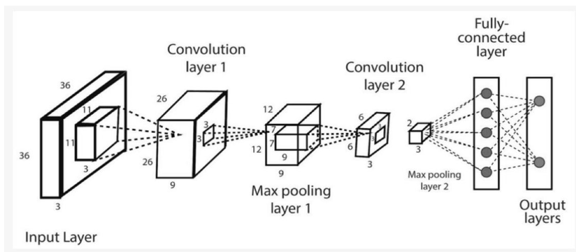
Figure 1. Convolutional Layer
