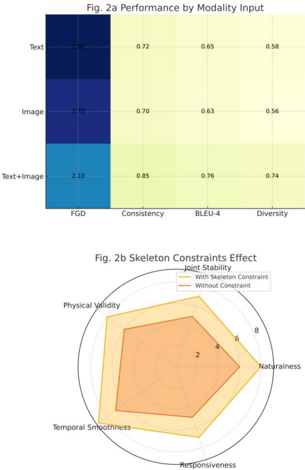
Figure 2. Evaluation of motion quality, diversity, and temporal consistency.
