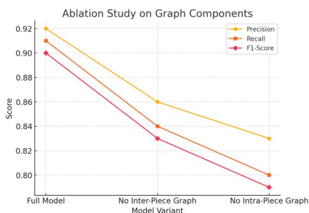
Figure 2 illustrates the impact of different graph modules on performance, using precision, recall, and F1-score metrics.
