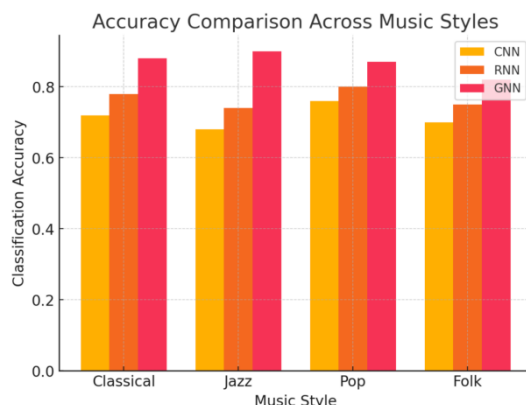
Figure 1 presents a comparison of classification accuracy across different music styles and model architectures, highlighting the superior performance of the GNN-based framework.
